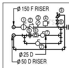
DETAIL FLOOR CONTROL VALVE
